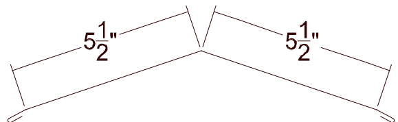
RESIDENTIAL RIDGE/HIP FLASH RR-1
