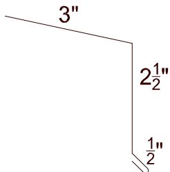
RESIDENTIAL GABLE WG-1
