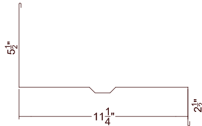
SOFFIT BOX - SOLID AB-3 WHITE VENTED AVAILABLE
