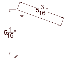
"Monoslope Ridge Flashing"
