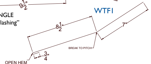
"Transition Flashing"
