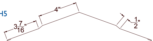
"Standard Ridge Flashings"
