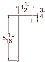
"Gable Flashing"
